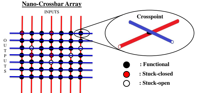
Fig. 1. Nano-crossbar array with faulty/defective crosspoints.
